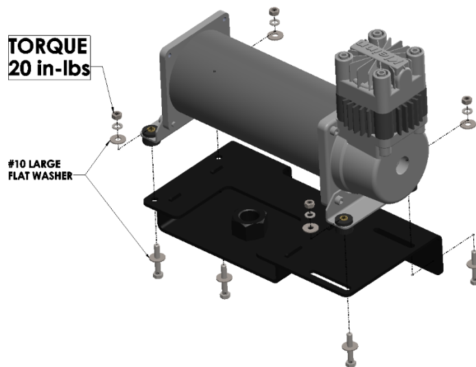
Figure 9- Compressor-to-Bracket Installation
