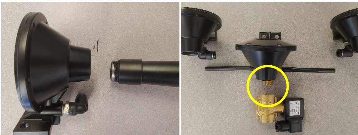
Figure 5- Trumpet Removal & Solenoid Installation
