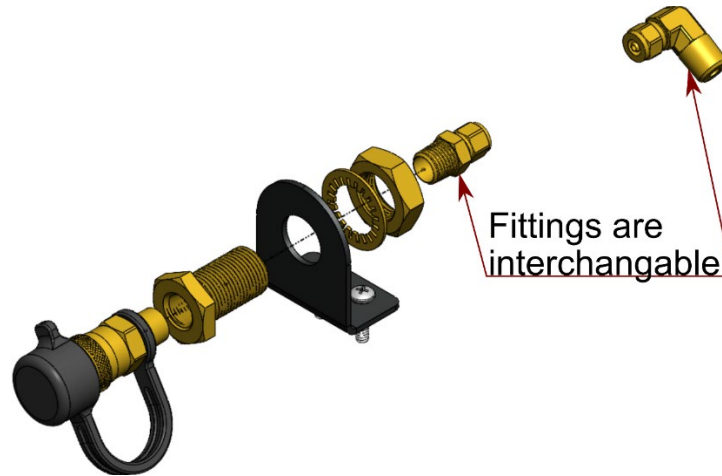
Figure 23- 1302 Quick Connect Kit, Assembly View
