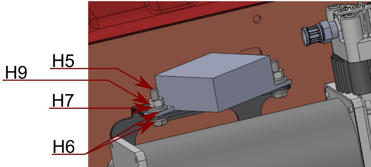
Figure 13- Computer Module, Hardware Stacking Order
