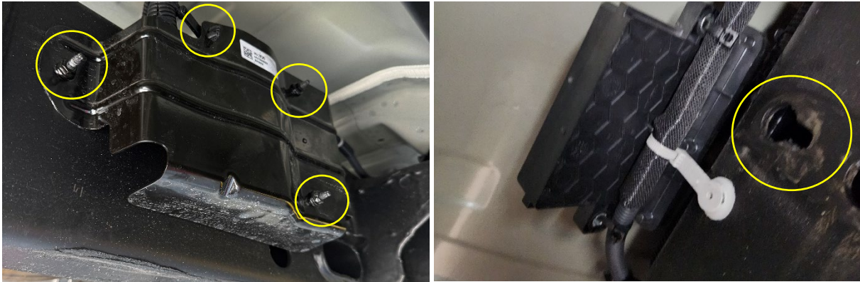
Figure 9- Module Shield Removal 1
