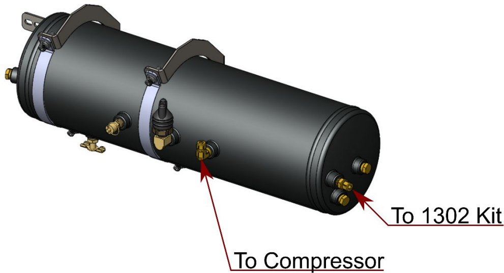
Figure 24- Final Plumbing of Air System
