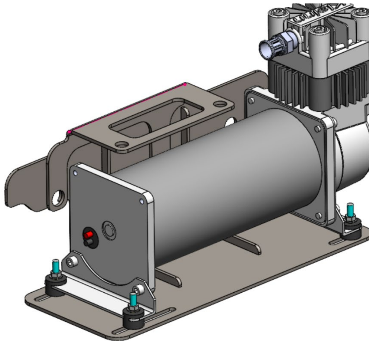
Figure 14- Compressor Mounted, Compressor & Hardware Orientation
