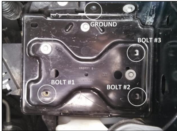
Figure 1: Battery tray prior to installation:
