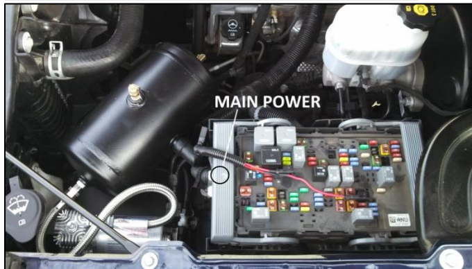
Figure 3: Remote Filter Mount Behind Fusebox:
