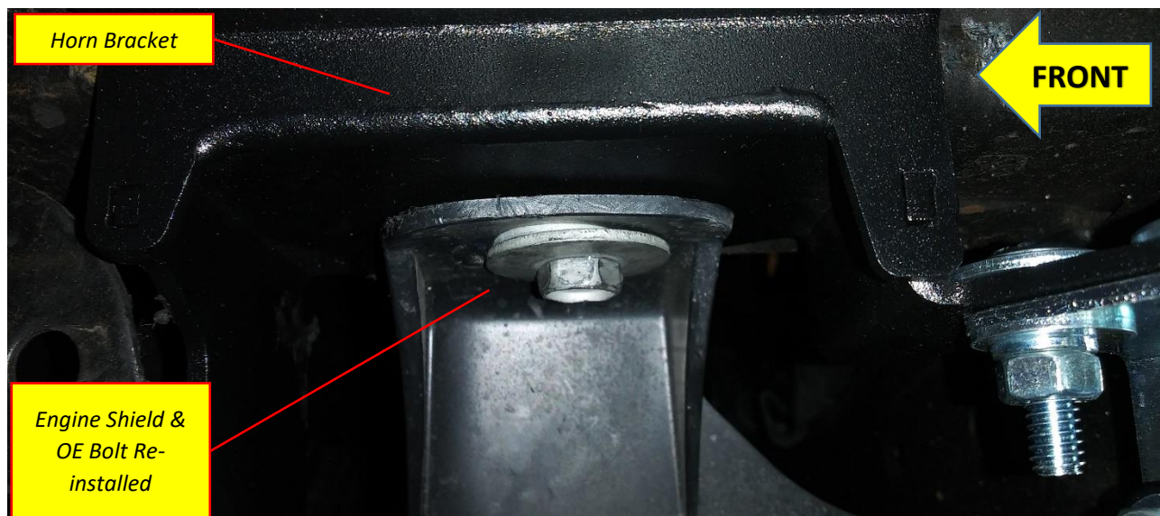
Figure 29 – Air Horn Sub-Assembly installed with Engine Shield in place (2020 Silverado Shown)
