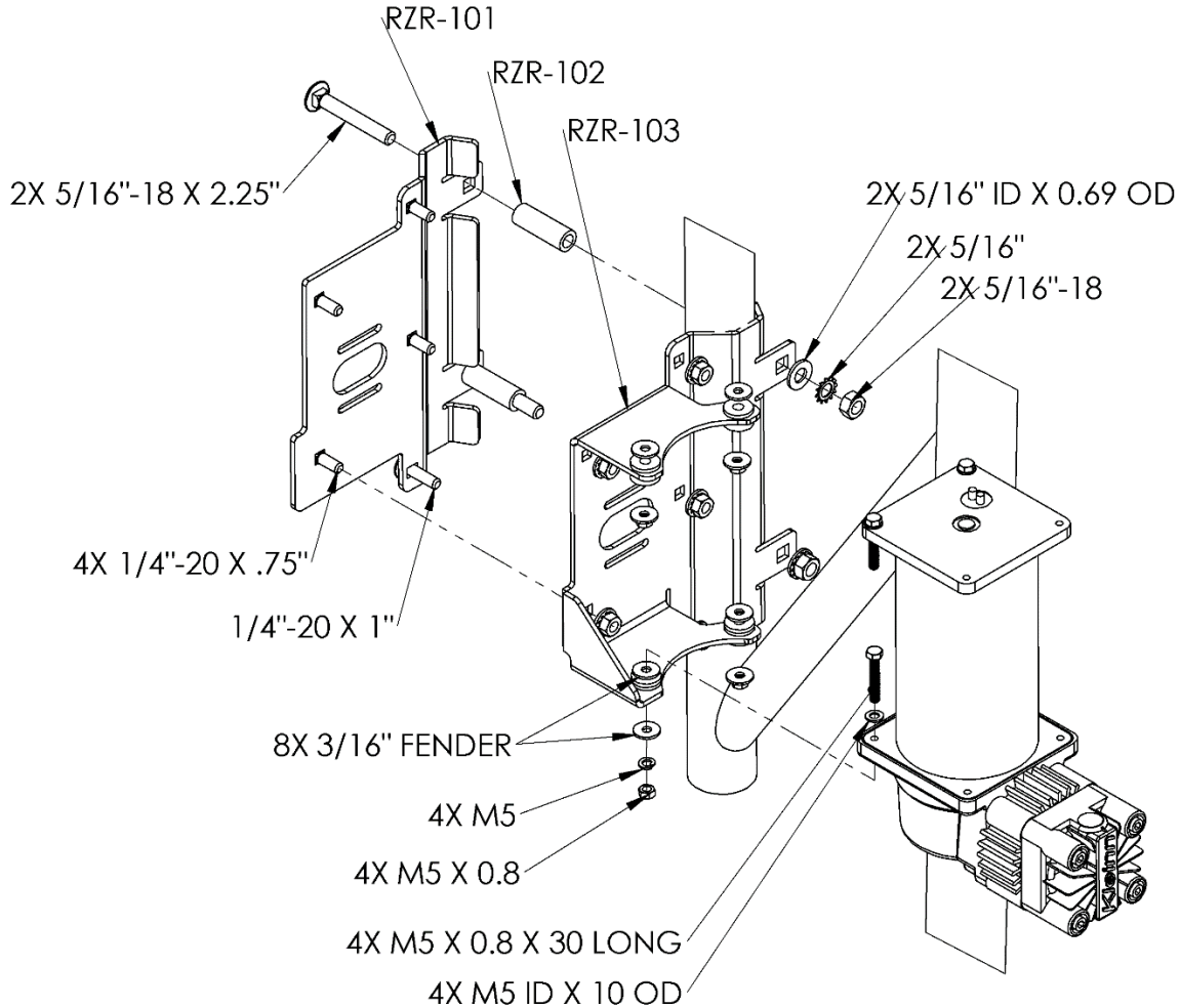
Figure 16 - Air Compressor Assembly & Hardware Exploded View
