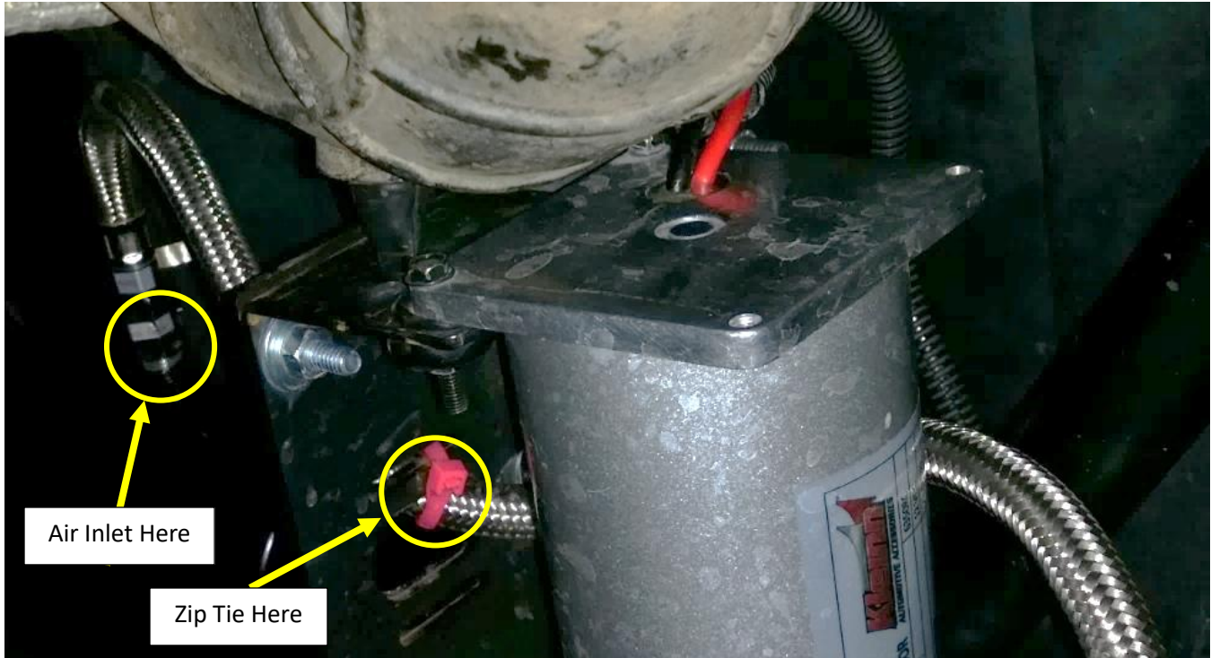
Figure 23 - Air Compressor Final Install with Leader Hose Connection to Air Tank
