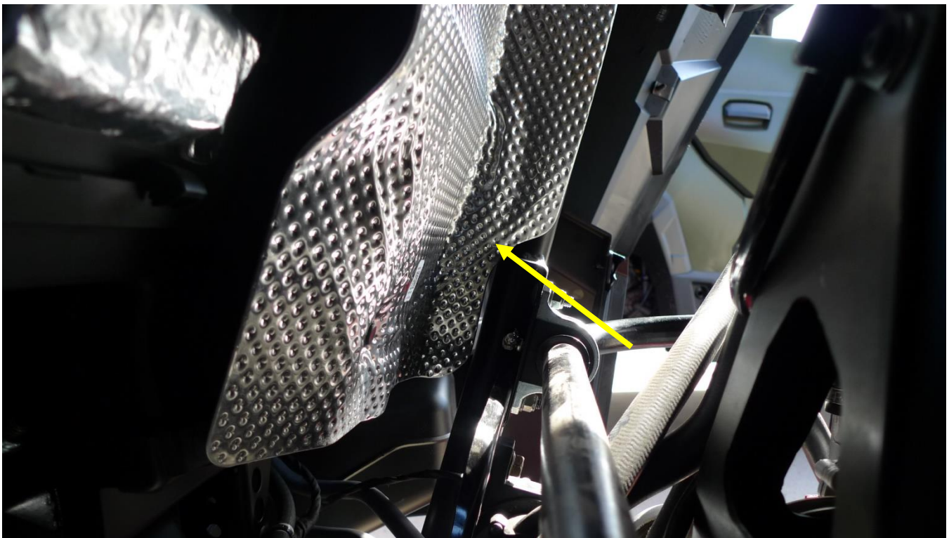
Figure 10 - Firewall Heat Shield, to Remove (Turbo Only)
