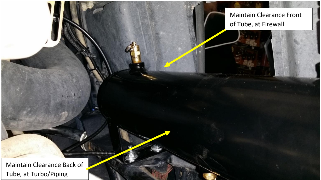
Figure 18 - Air Tank to Vehicle Clearance
