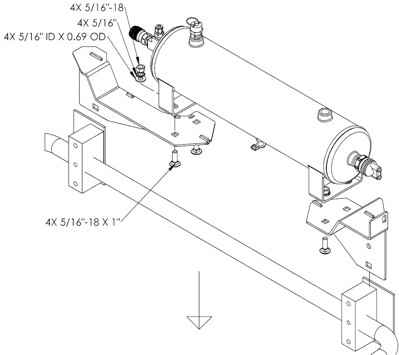
Figure 17 - Air Tank and Air Tank Brackets Exploded View
