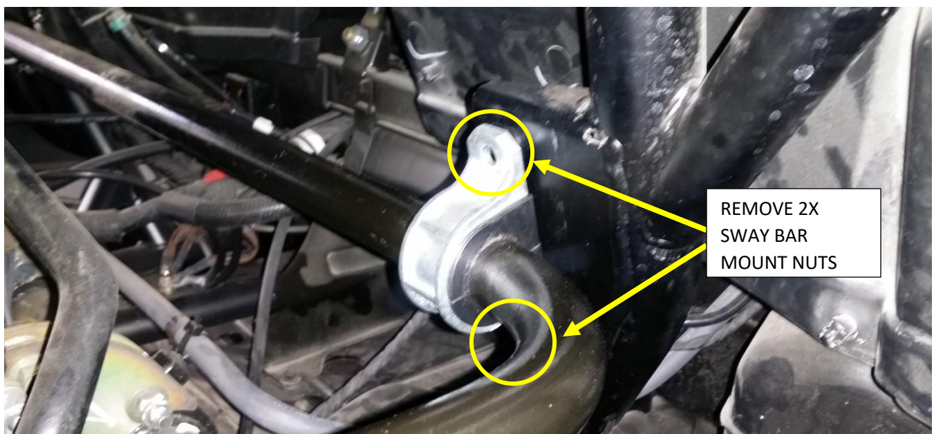
Figure 12 - Driver Side Sway Bar Nuts/Bolts, to Remove
