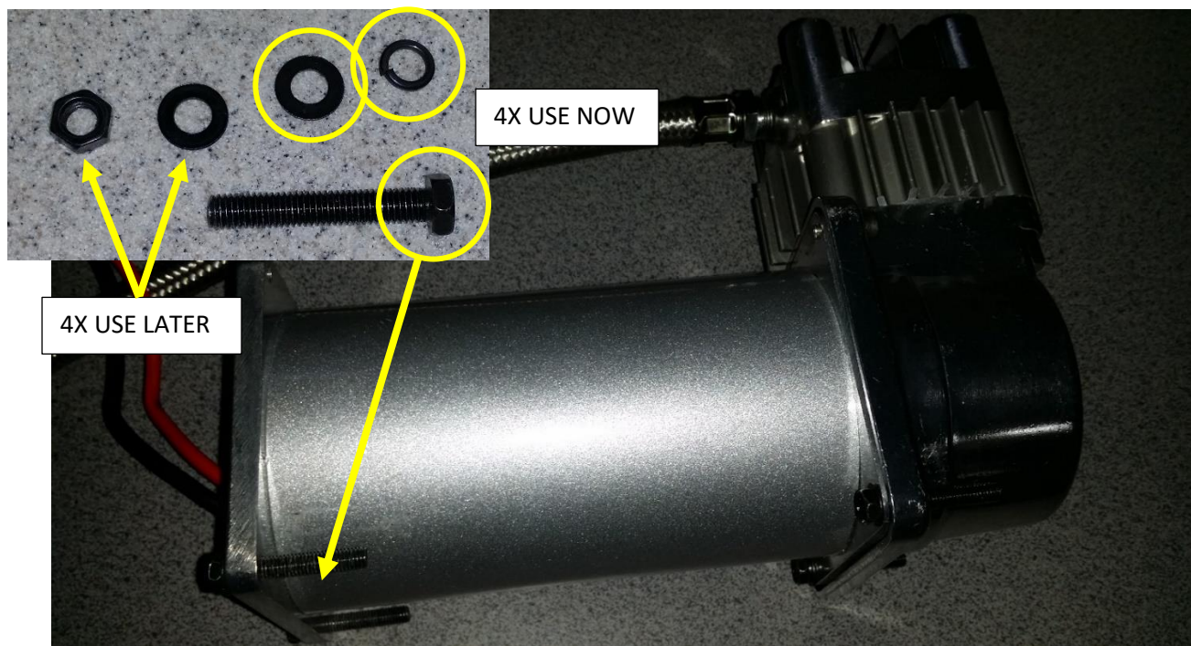
Figure 6 - Air Compressor with Bolts Installed as Studs
