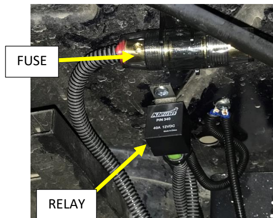
Figure 4 - Example of Relay and Fuse Mounted with Wire Loom
