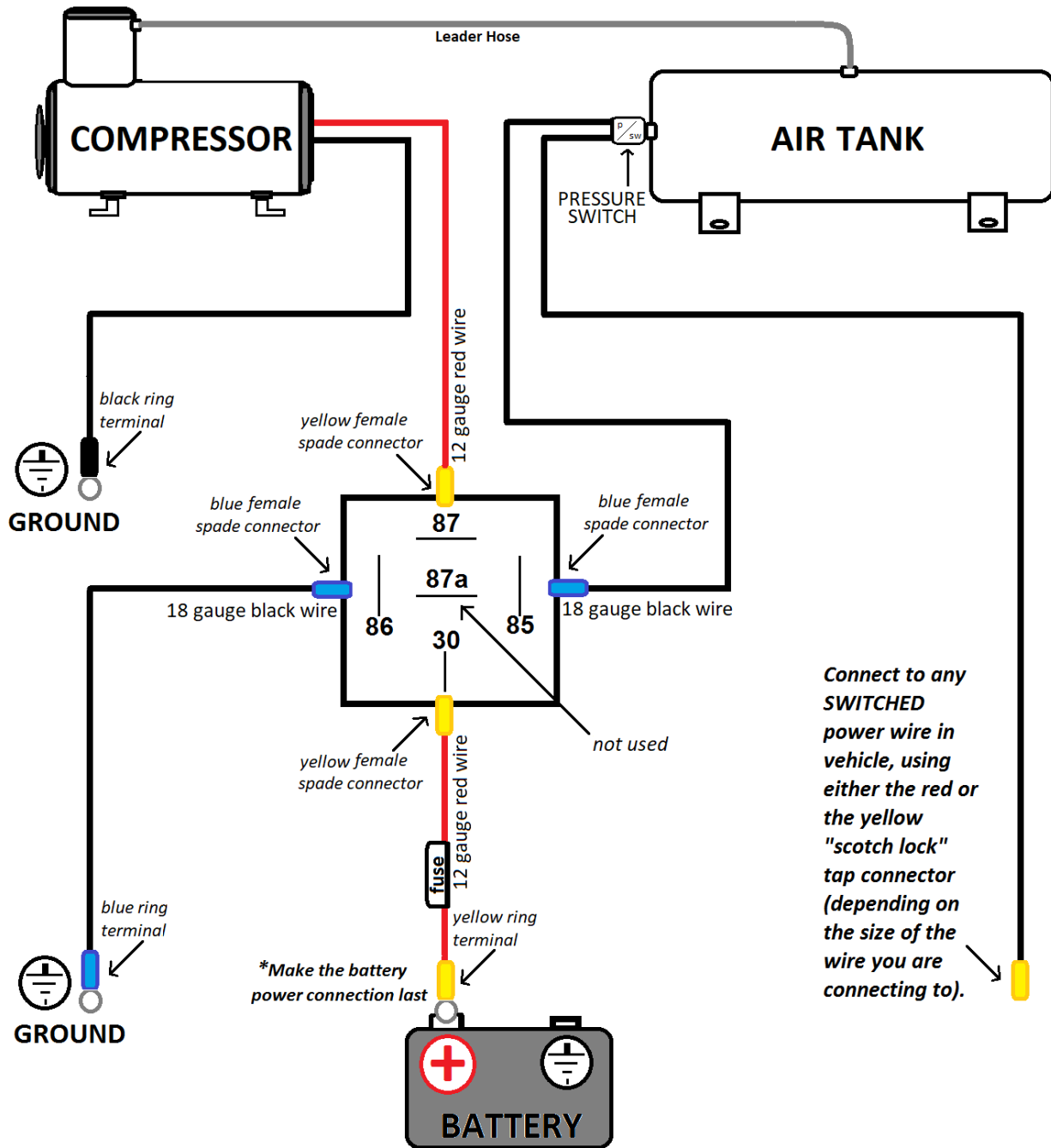
Figure 2 - Suggested Ignition Relay Diagram for Air Compressor and Air Tank
