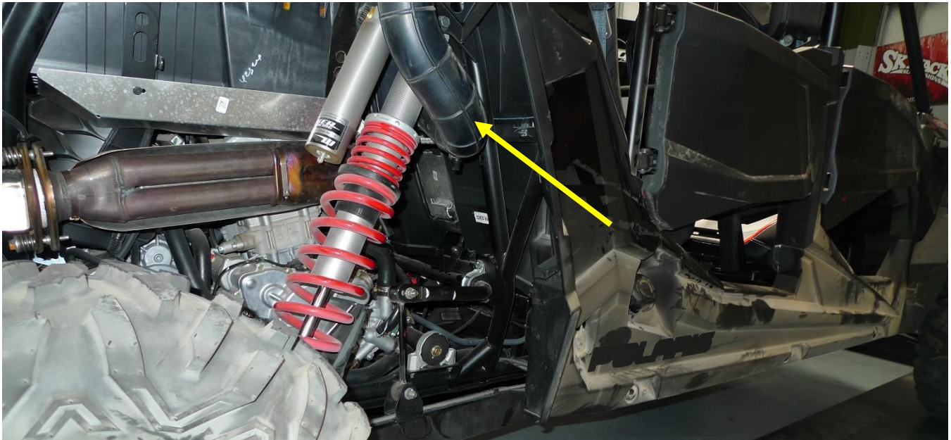
Figure 9 - Air Intake Tubing, to Remove
