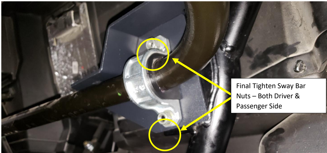
Figure 21 - Driver Side Sway Bar Final Torque of Nuts/Bolts
