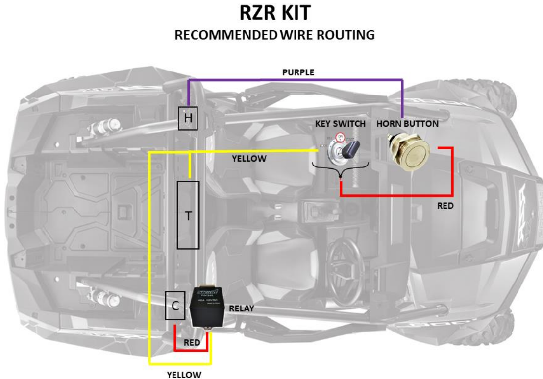
Figure 3 - Suggested Wire Routing for Horn, Air Compressor, and Pressure Switch
