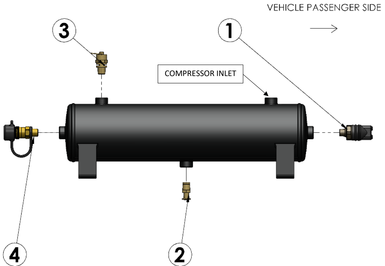
Figure 5 - Air Tank Exploded View
