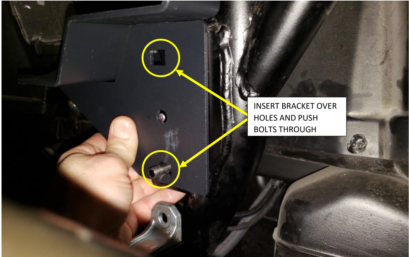
Figure 13 - Driver Side Air Tank Bracket Insertion
